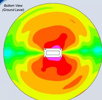
Acoustic Directivity
