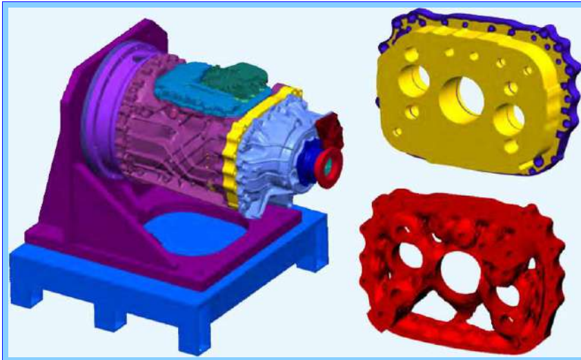
Topology optimization of a bearing support (by courtesy of ZF Friedrichshafen AG, Friedrichshafen)
