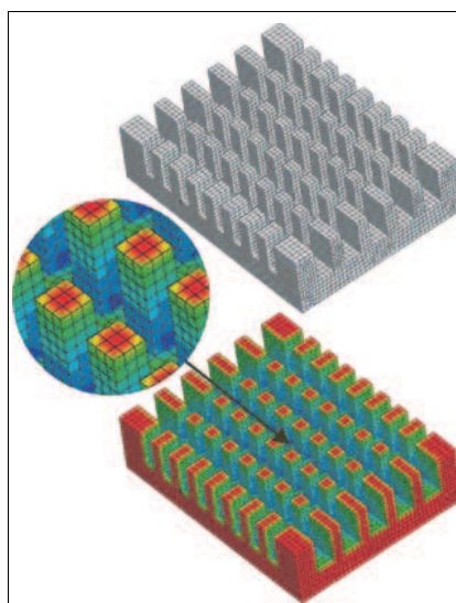
Analysis of cooling element with radiation
