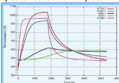
Temperature distribution over time with PERMASgraph
