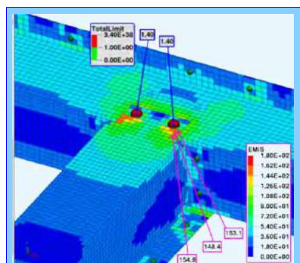
Evaluation of spot weld forces
