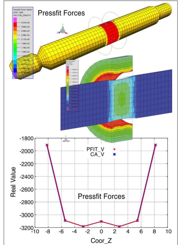
Figure 12: Press fit connection comparison of MPC and contact result
