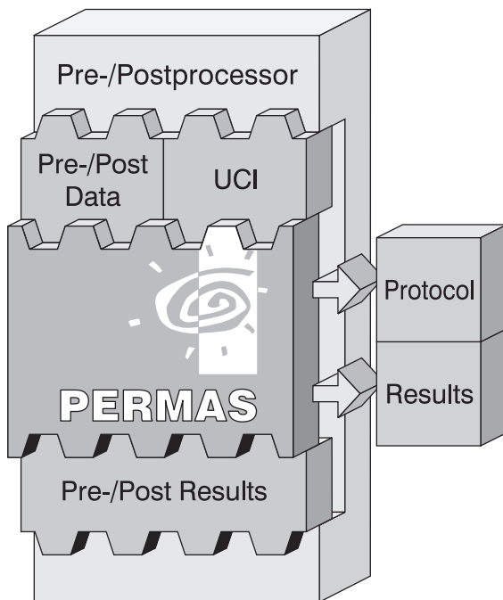
Figure 97: Integration of PERMAS in pre- and post-processor
