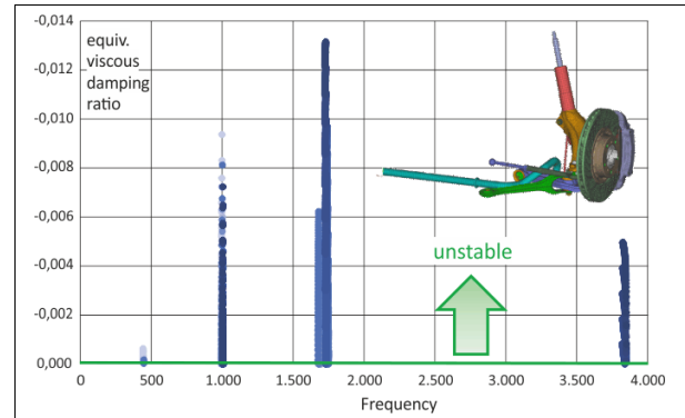
Figure 39: Stability map of a brake for 7110 parameter sets from rotational speeds, Young's modulus of disk, and frictional coefficient between disk and pad. The total run time for this stability map was 5 hours 12 minutes.
