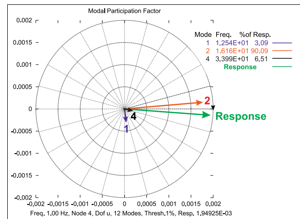
Figure 130: Modal grid participation factors
