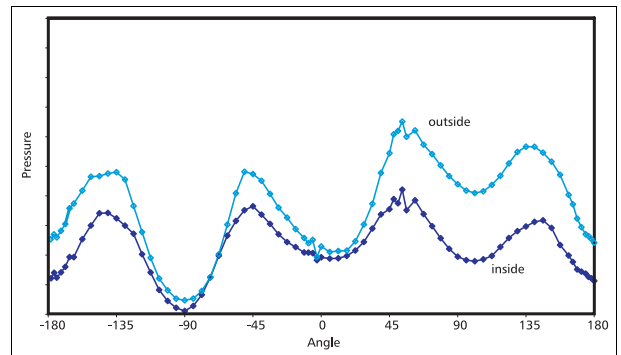
Figure 30: Pressure distribution at stopper over the angle
