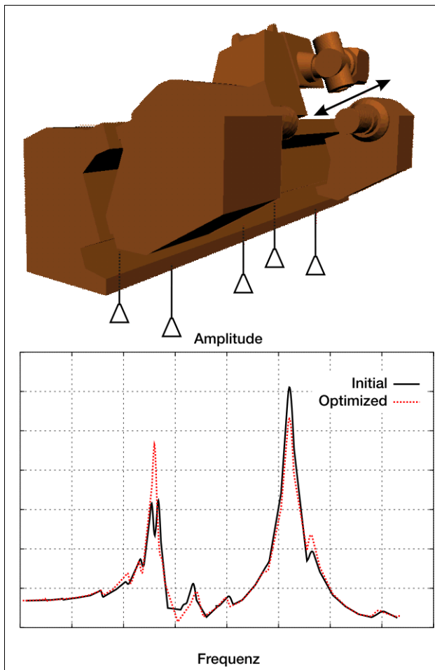
Figure 135: Frequency response optimization for a machine foundation where the position of the base spring elements is optimized which are coupled to the machine structure by interpolating surfaces. Design objective is the maximum flexibility of the tool center point.
