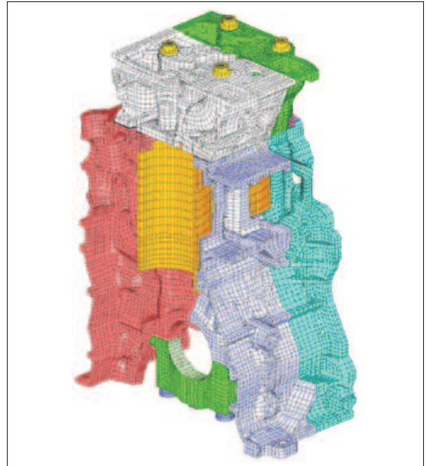
Figure 28: Simple engine model Daimler AG, Commercial Vehicle Division)
