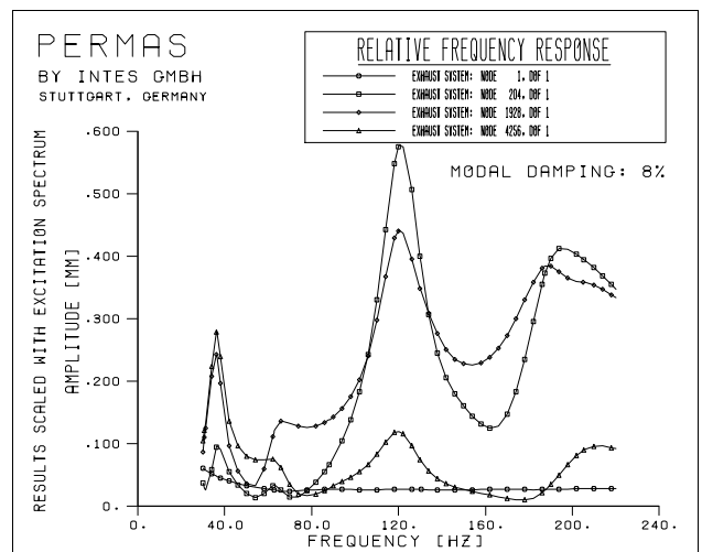
Figure 151: Exhaust System Frequency response analysis
