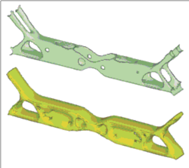
Figure 140: Different results for topology without (above) and with (below) release directions
