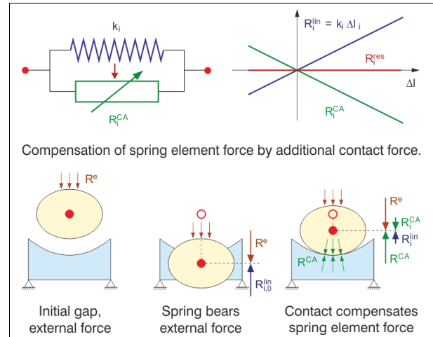
Figure 107: Force-guided contact with the aid of compensation spring
