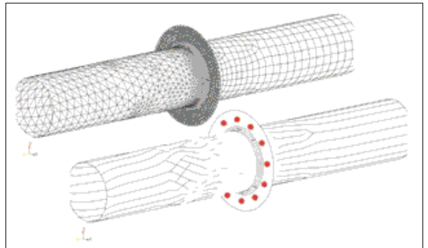
Figure 85: Spotwelds and incompatible meshes
