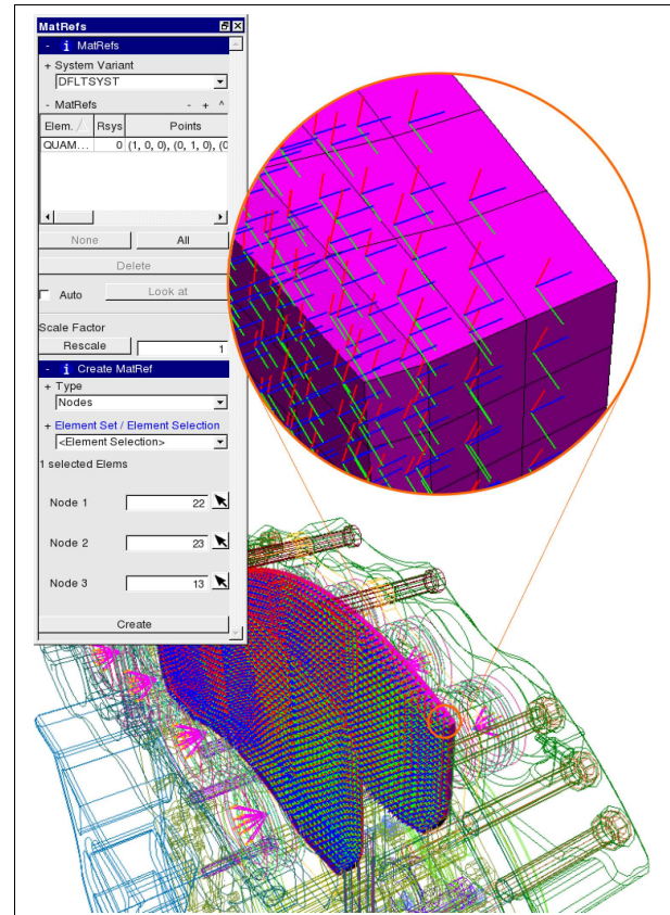
Figure 19: Material reference system for anisotropic material
