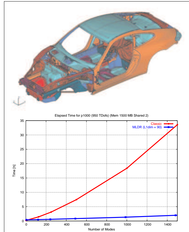
Figure 127: Comparison of elapsed run times for Subspace Iteration (upper curve) and MLDR (lower curve) with increasing number of modes (157412 Nodes, 164301 Elements (QUAD4), 944472 Unknowns)
