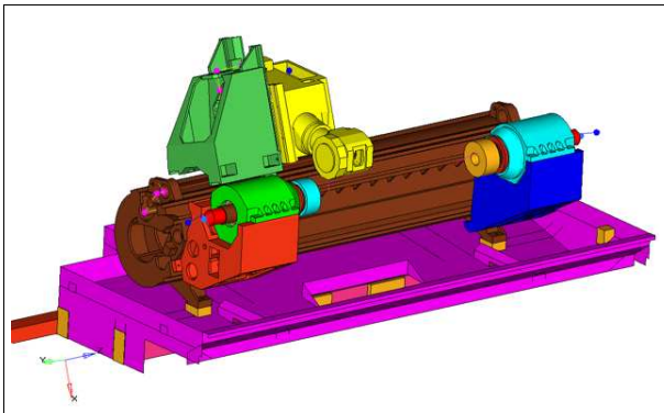
Figure 22: Machine tool INDEX-Werke GmbH & Co. KG, Esslingen, Germany
