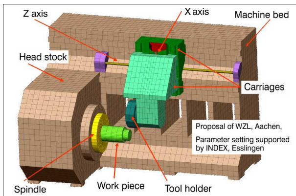
Figure 42: Simplified model of a turning machine as proposed by WZL in Aachen and supported by INDEX, Esslingen for setting suitable parameters
