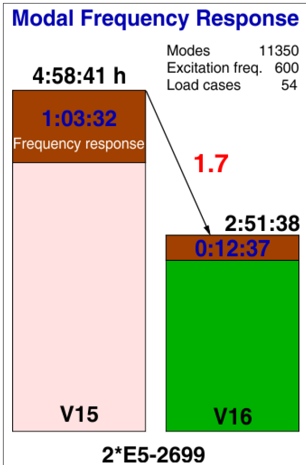
Figure 8: Modal frequency response analysis with high run time savings.
