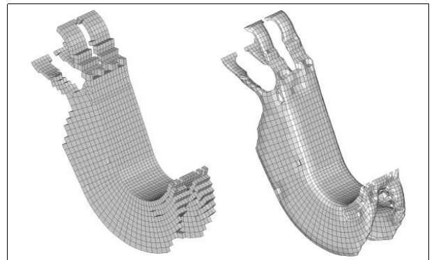
Figure 143: Layout-Optimization of a crane hook (on the left side the primary result, on the right side the smoothed surface)
