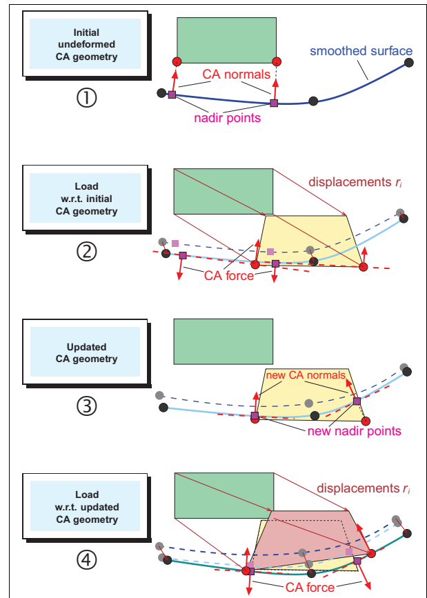
Figure 114: First steps in contact update
