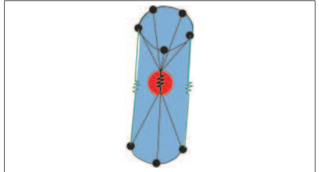
Figure 84: Spring element at spotweld position
