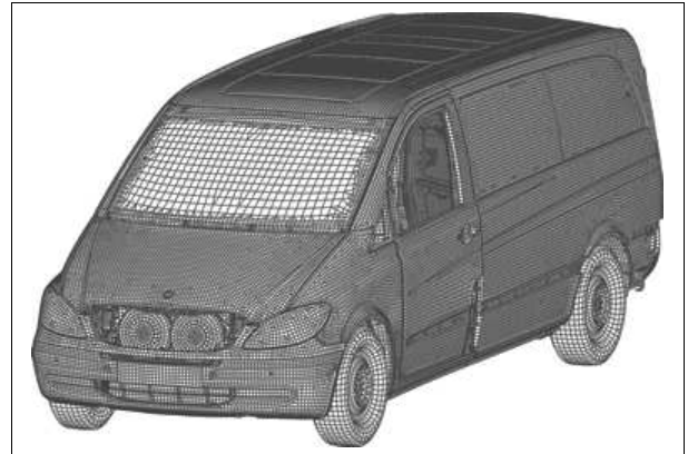
Figure 21: Model of a transport vehicle courtesy of Daimler AG, Commercial Vehicle Division in Stuttgart
