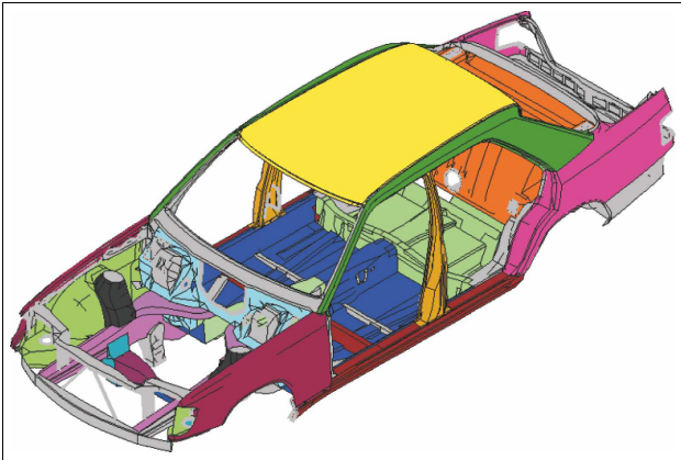
Figure 134: Frequency response optimization of a body-in-white with shape and sizing parameters (see also Fig. 137)
