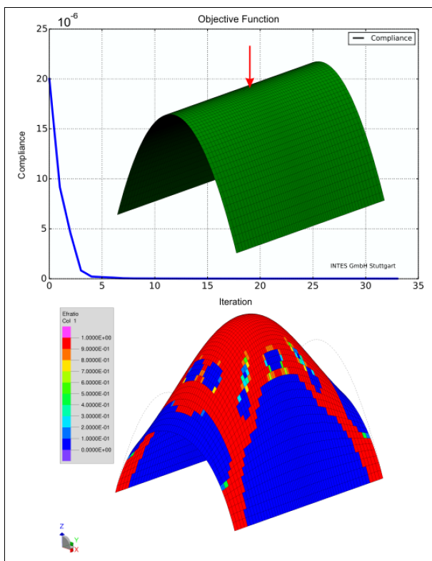
Figure 17: Topology and shape optimization simultaneous solution as multi-modal optimization
