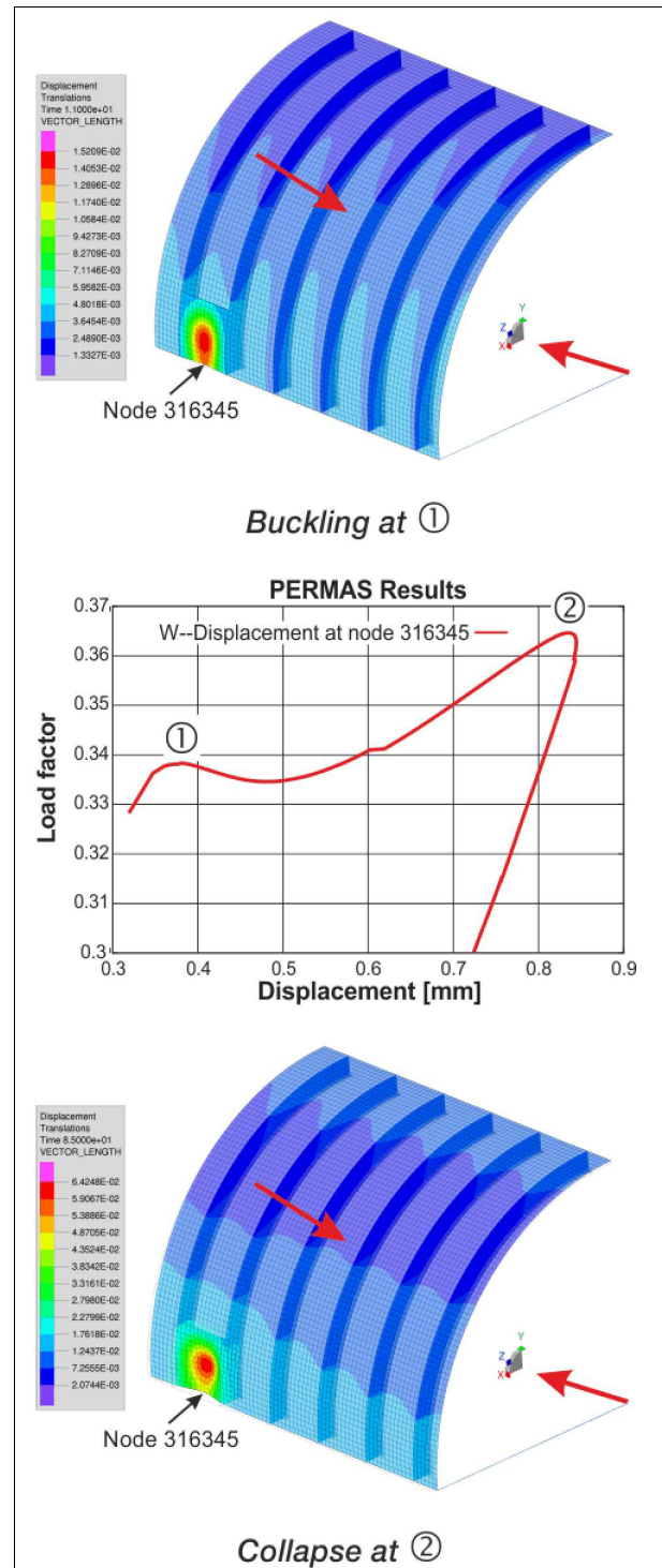
Figure 116: Elastic-plastic buckling with post-buckling behavior
