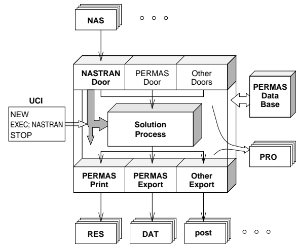
Figure 153: UCI trigger for NASTRAN-Task
