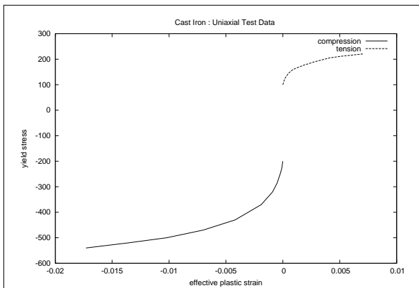
Figure 119: Uniaxial test data of a cast iron material
