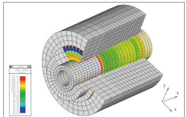
Figure 110: Conical press fit (slipping forces after assembly)
