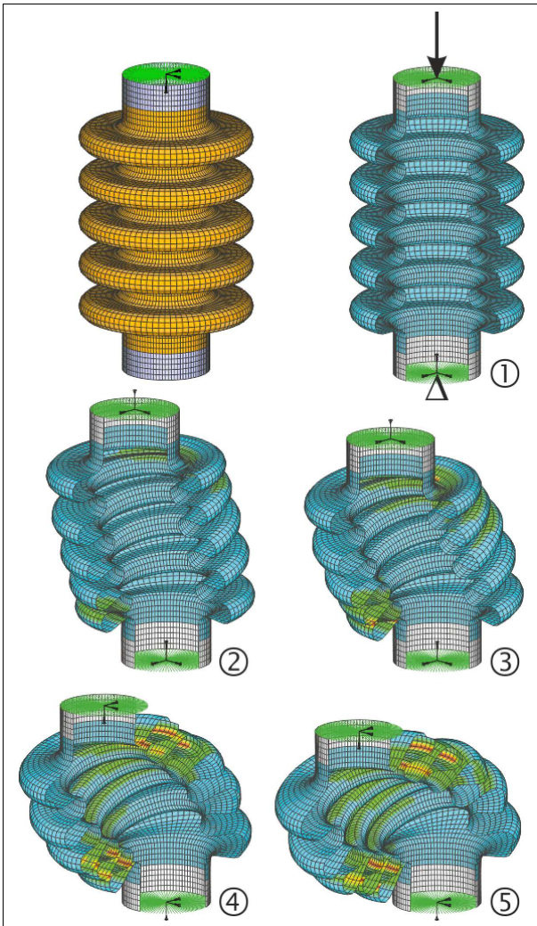
Figure 111: Self contact of a bellow
