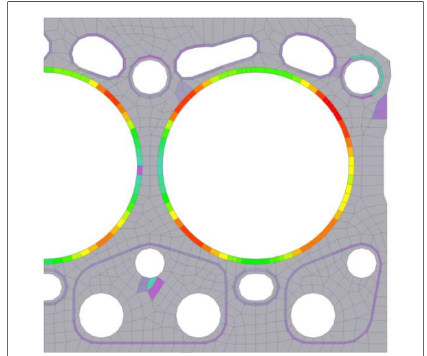
Figure 117: Pressure of cylinder head gasket
