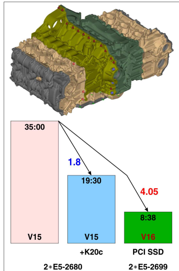
Figure 9: Direct I/O for large models with PCI SSD like contact analysis of engine with 56 Million DOF, 37 time steps, 2 different temperature states, and CAS files, including GPU.
