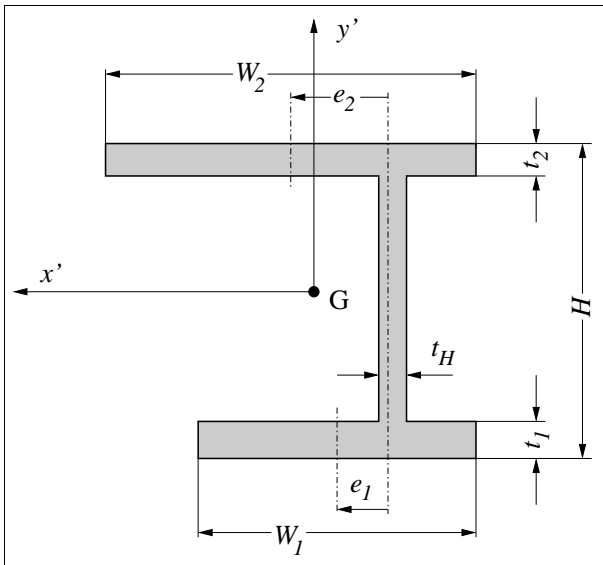
Figure 91: General thin-walled open section
