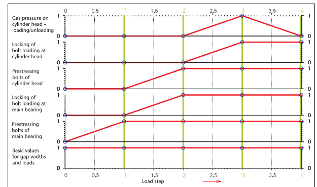
Figure 105: Representation of a load history
