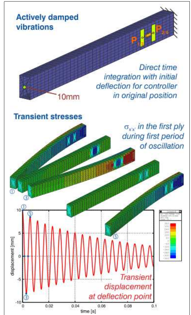
Figure 48: Active damping of a composite box girder
