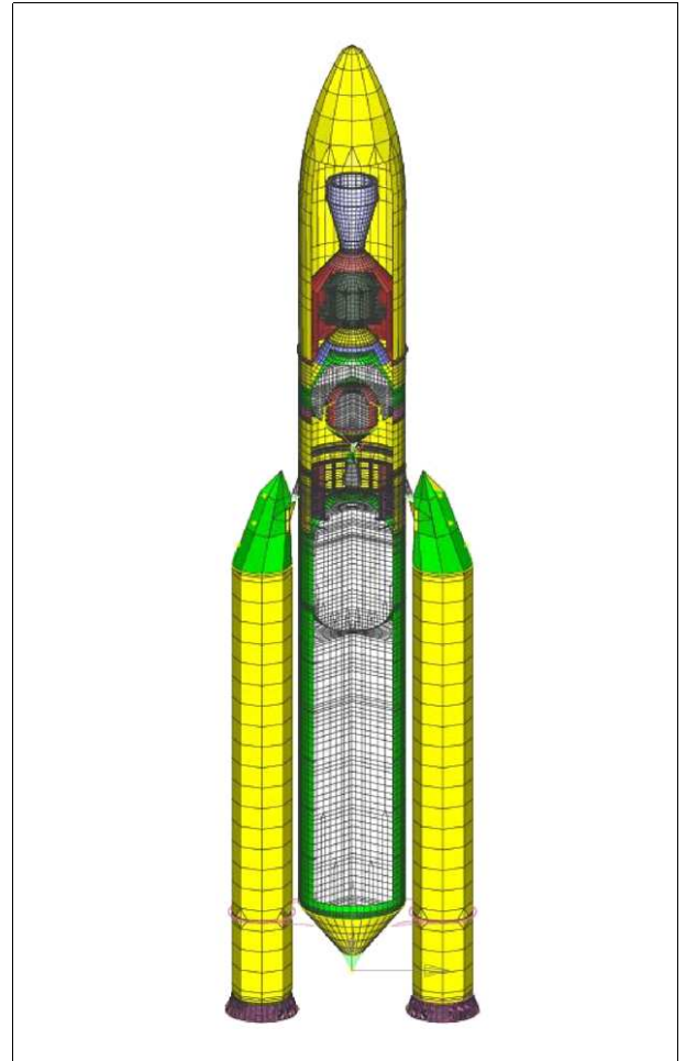
Figure 126: Ariane 5 launcher model by courtesy of ASTRIUM Space Transportation, Les Mureaux
