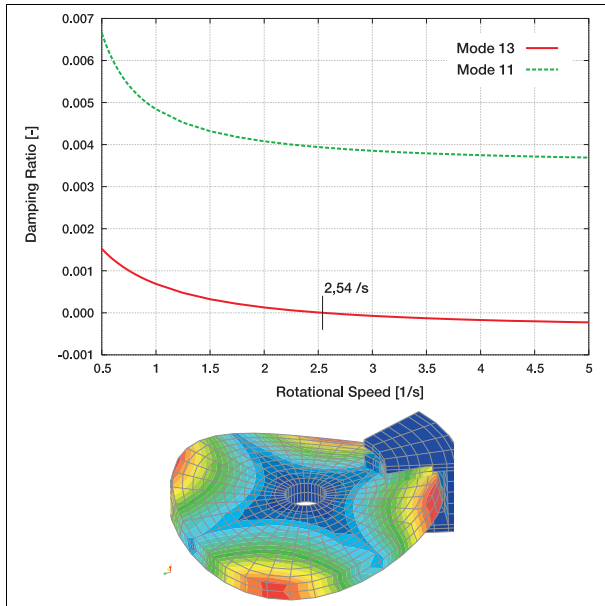
Figure 35: Simple brake model (1) with an unstable bending mode ( m=2, n=1 ) at 2,54 rps
