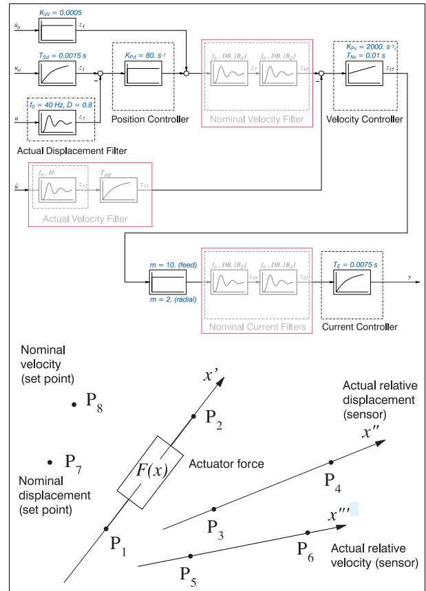
Figure 43: Block diagram of used controller and corresponding finite element representation
