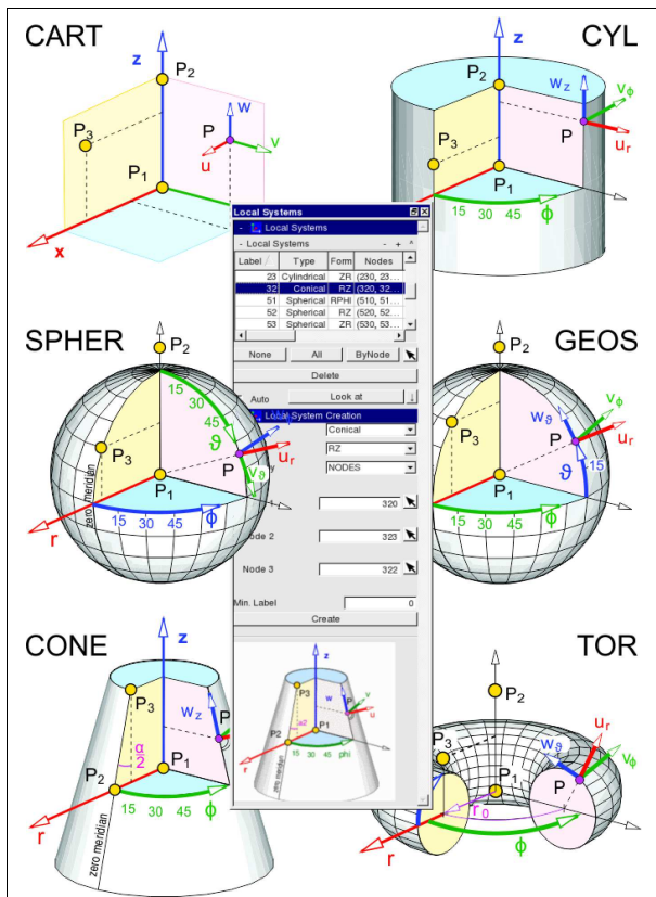
Figure 87: Local coordinate systems in VisPER
