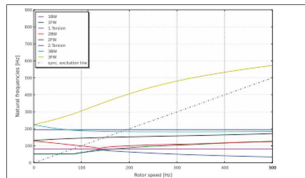
Figure 40: Campbell diagram for the evaluation of rotor dynamics
