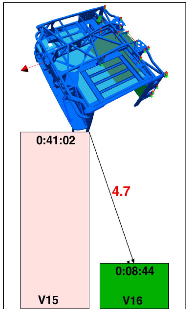
Figure 15: Run time reduction in geometrically nonlinear analysis for a 3 Million DOF frame structure (in minutes)
