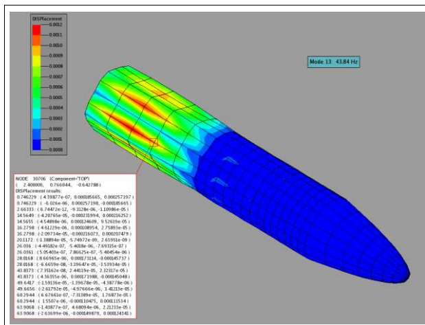
Figure 69: Display and animation of mode shapes on full substructure model
