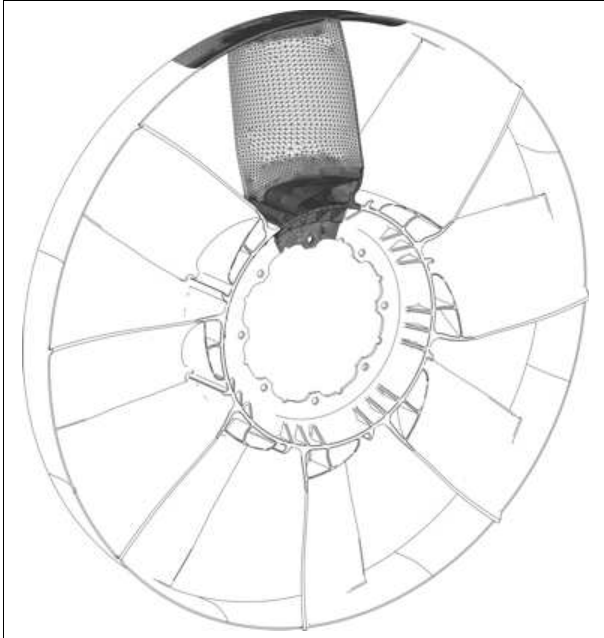
Figure 76: Cyclic symmetry of a fan Behr GmbH & Co., Stuttgart, Germany.
