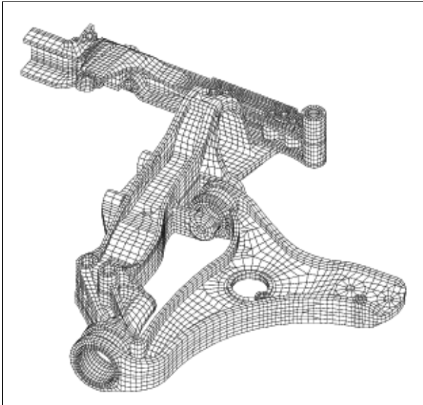
Figure 102: Model of a front axle Porsche AG, Weissach
