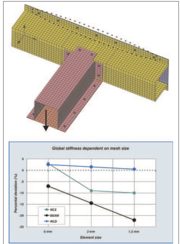
Figure 149: Quality of the refined weldspot model
