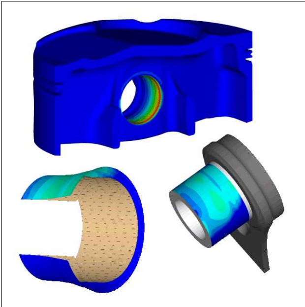
Figure 146: Optimization of contact pressure between piston and piston pin (Mahle GmbH, Stuttgart). The figure shows the optimized geometry of the piston and the reduced edge pressure.
