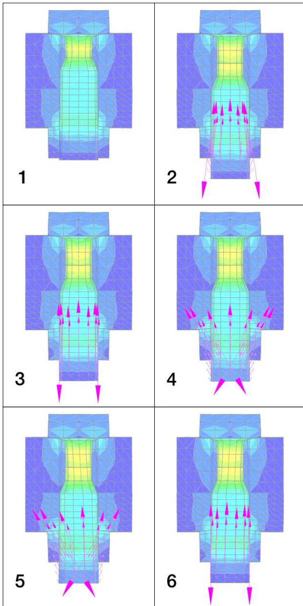
Figure 106: Bolt pretension Nodal point stresses and pretension forces for deformed mid-size screws:
