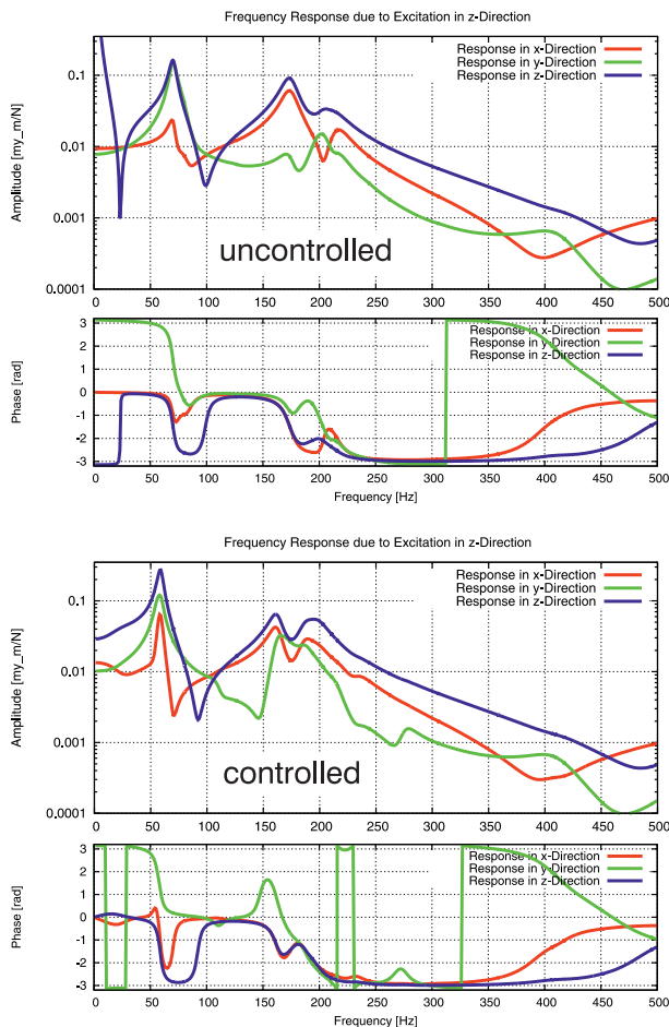
Figure 44: Frequency response between tool and workpiece due to excitation in Z direction for uncontrolled (above) and controlled (below) machine
