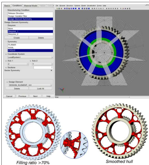
Figure 58: Topology optimization of a gearwheel Definition of cyclic symmetry and release directions, max. stress at interface between design space and gear rim, max. allowed weight, minimum compliance as objective function (by courtesy of Daimler AG, Stuttgart).
