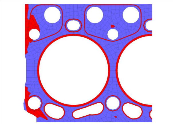
Figure 29: Contact status for gasket elements
