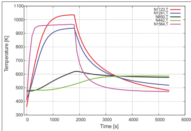
Figure 120: Transient temperatures at nodes over time
