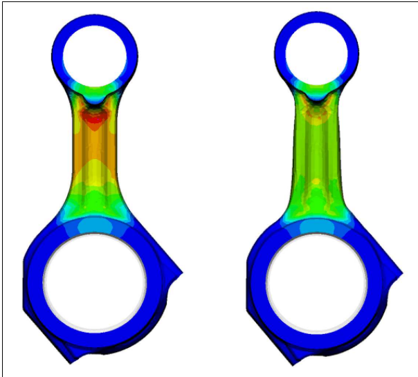
Figure 138: Stress homogenization of conrod
