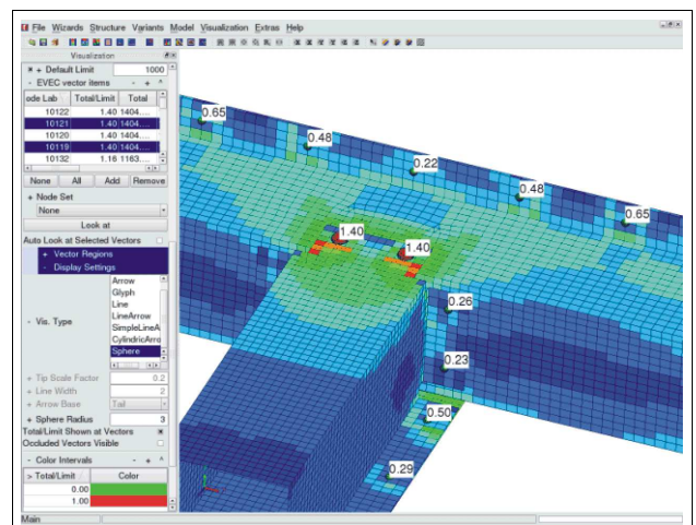
Figure 70: Evaluation of spotweld forces together with element stresses
