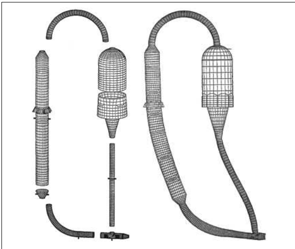
Figure 93: Mode shape of a reactor
