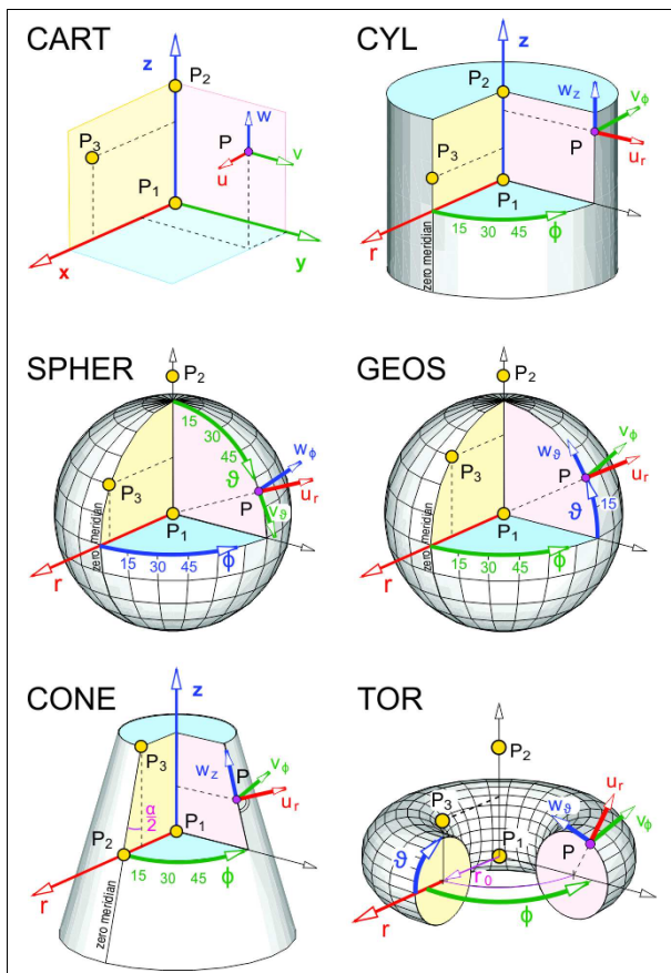
Figure 11: Local coordinate systems
