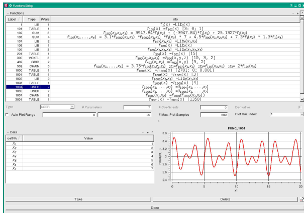
Figure 94: Functions dialogue in VisPER
