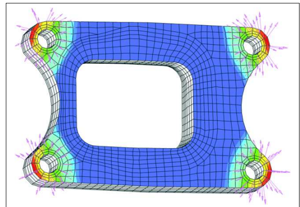
Figure 108: Contact pressure and shear vectors
