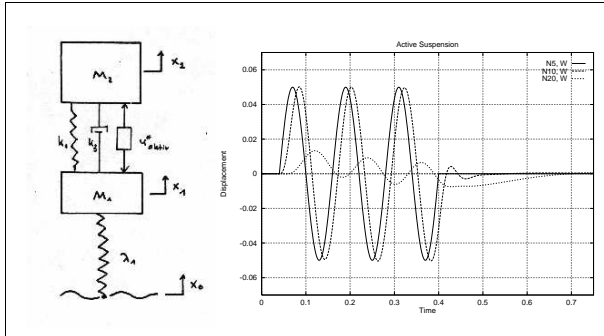
Figure 49: Active suspension unit
