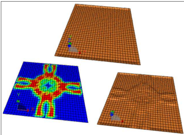
Figure 27: Bead design of a plate with positioning and height of beads
