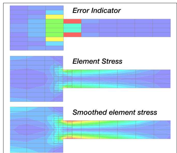
Figure 92: Example for error indicator , element stress , and smoothed element stress
