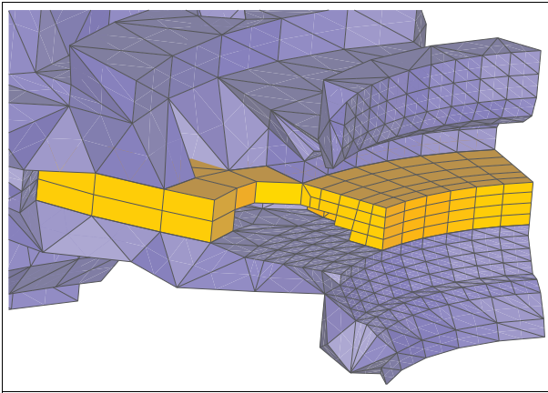
Figure 78: Incompatible meshes Element transition (HEXE8/TET10)
