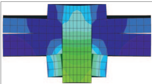
Figure 33: Short bolt under pretension
