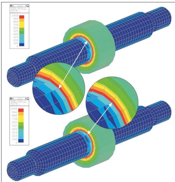
Figure 89: Press fit between shaft and hub Identical stress results of MPC (above) and contact solution (below).
