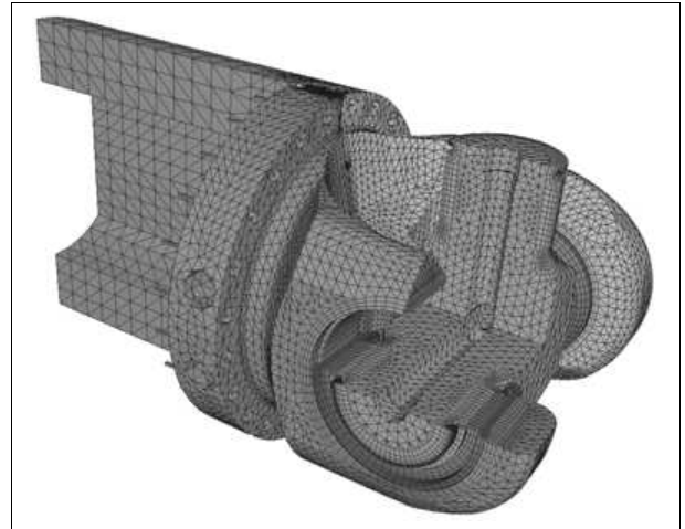
Figure 77: Incompatible meshes Cardan shaft model in sectional view (Voith Turbo GmbH & Co. KG)
