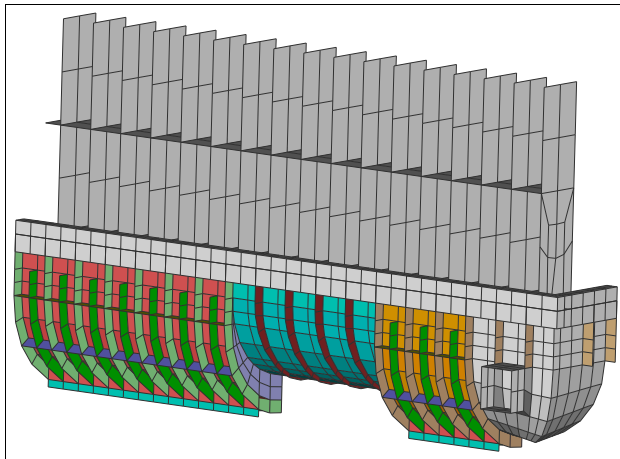
Figure 50: Optimization of a water box with 18 design variables and 19 stochastic basic variables
