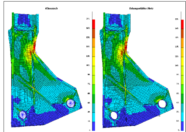
Figure 79: Ribbed shell model with compatible meshes (left) and incompatible meshes (right)
