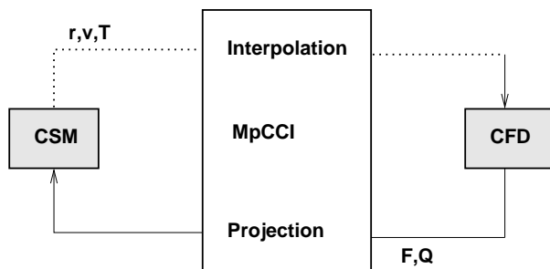
Figure 101: Coupling of CFD and CSM
