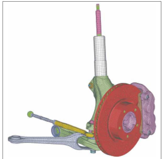
Figure 34: Brake model
