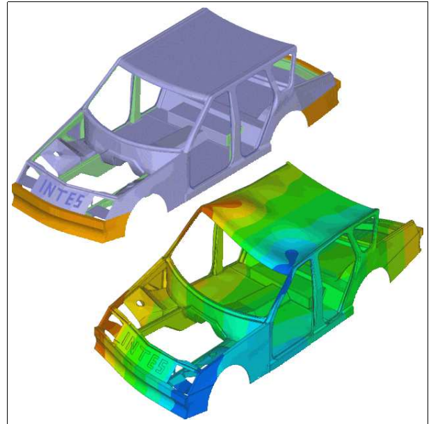
Figure 25: Workshop example INTEScar under torsional loading
