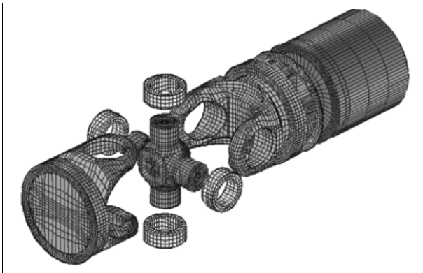
Figure 24: Model of a cardan shaft
