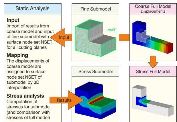
Figure 72: Submodeling in static analysis
