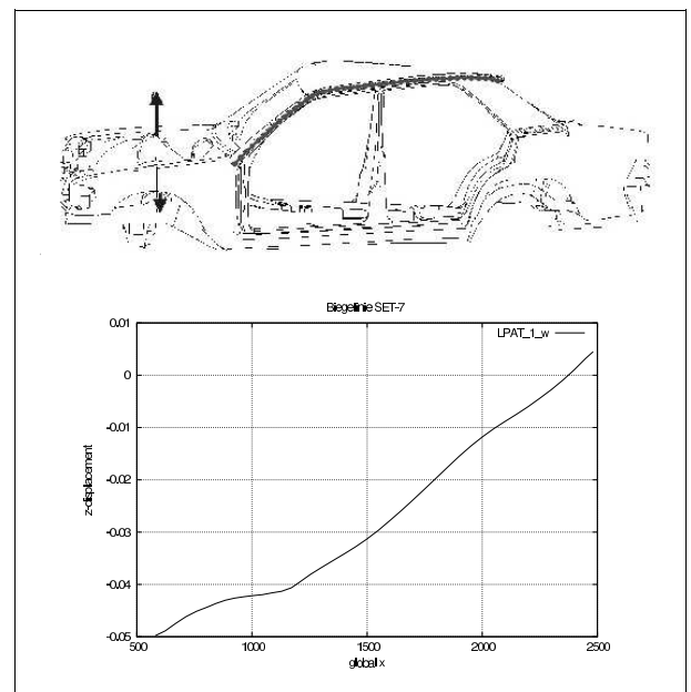
Figure 98: Determination of elastic line for torsional load case (displacement for the marked nodes)
