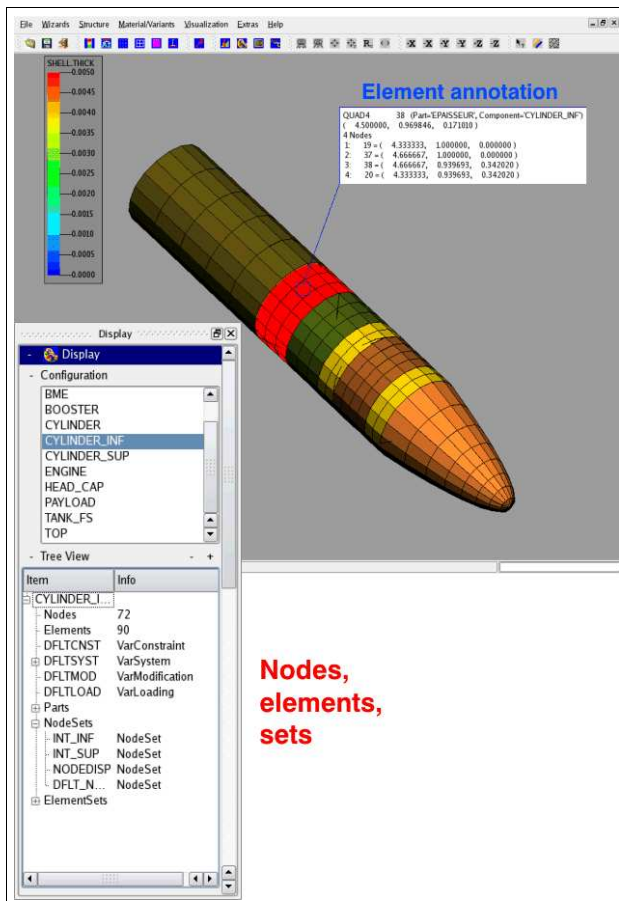
Figure 68: Checking element properties in a substructure model
