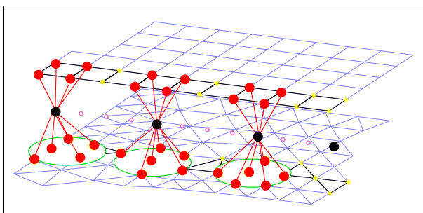
Figure 83: Connection of spotweld forces
