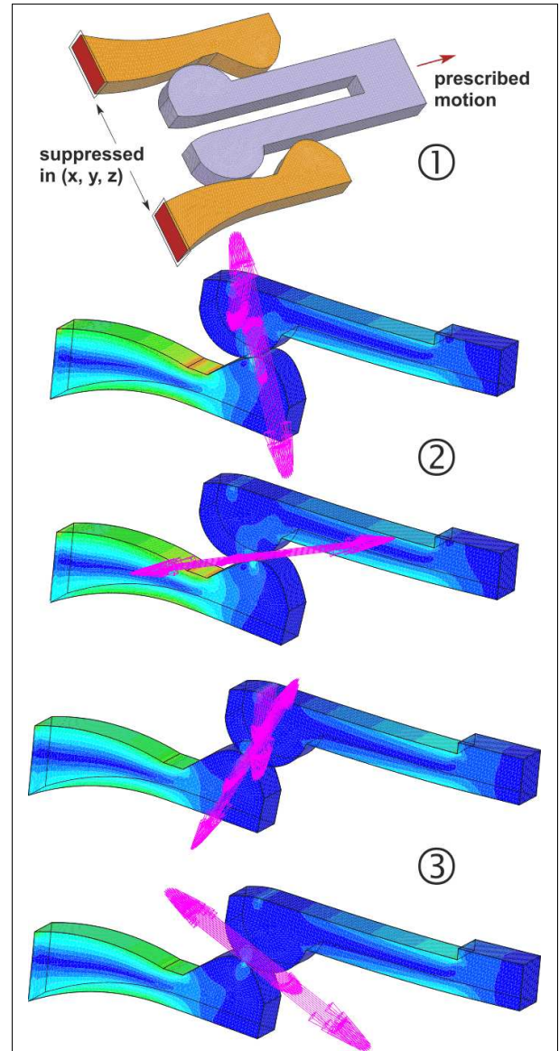
Figure 112: Clip example for contact update Large relative motion with friction. Picture 1 shows the model; pictures 2 show the contact pressure (above) and the frictional shear (below) with nodal point stresses before the bottleneck is reached; pictures 3 show the contact pressure (above) and the frictional shear (below) with nodal point stresses after the bottleneck is passed.
