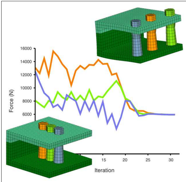
Figure 82: Shape optimization with incompatible meshes to achieve smallest relative displacements and identical bolt forces (top: initial design, bottom: final design; in between: bolt forces for each iteration)
