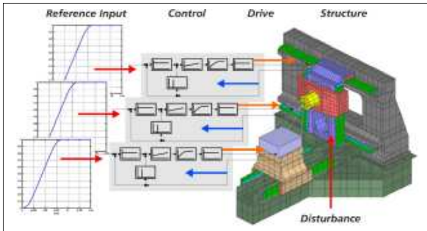
Figure 47: Principles of coupled analysis with control
