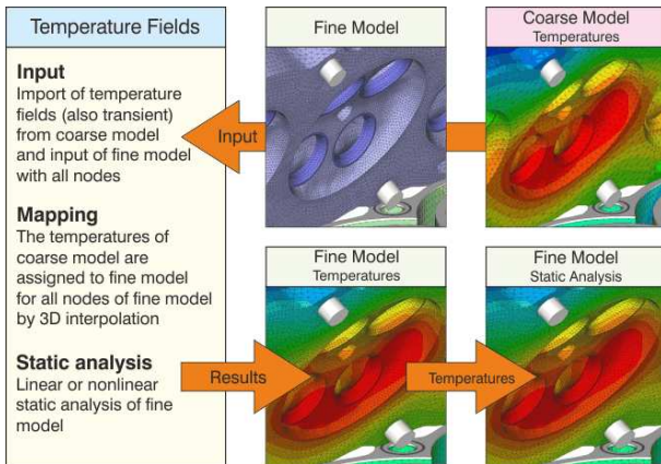
Figure 73: Mapping of temperature fields
