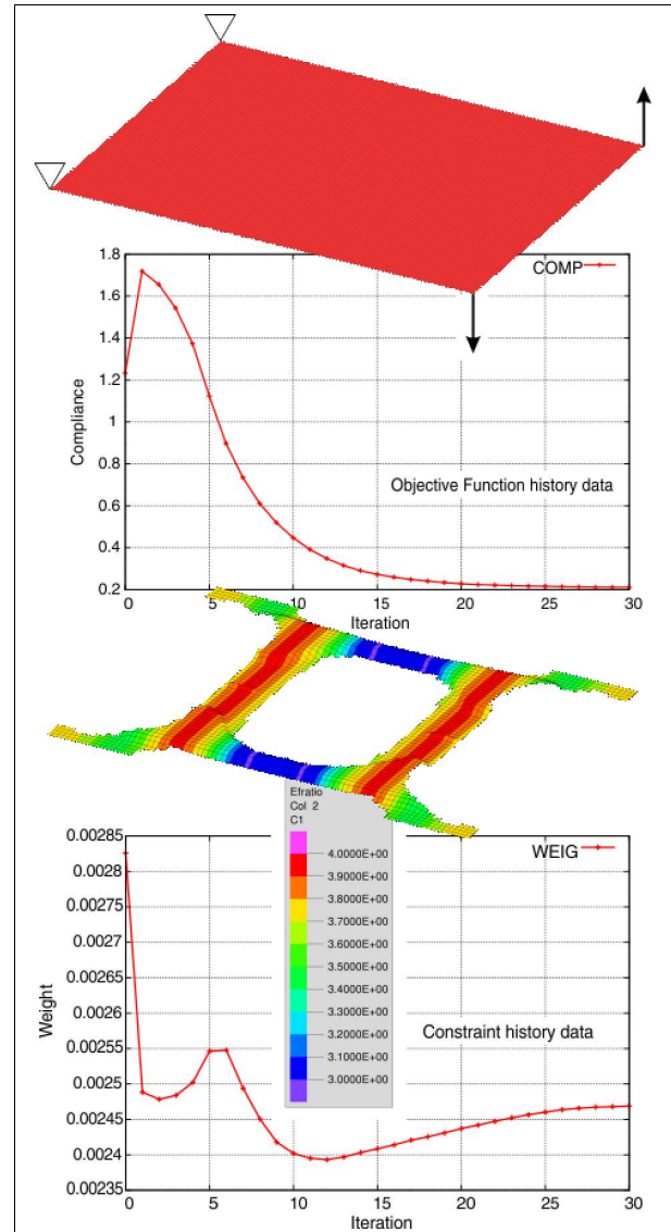
Figure 16: Multi-modal optimization with topology optimization, bead optimization, and free sizing for the sheet thicknesses.
