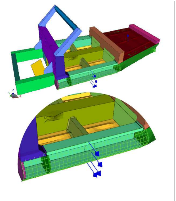
Figure 26: Shape optimization of a sill with transition to neighbored parts
