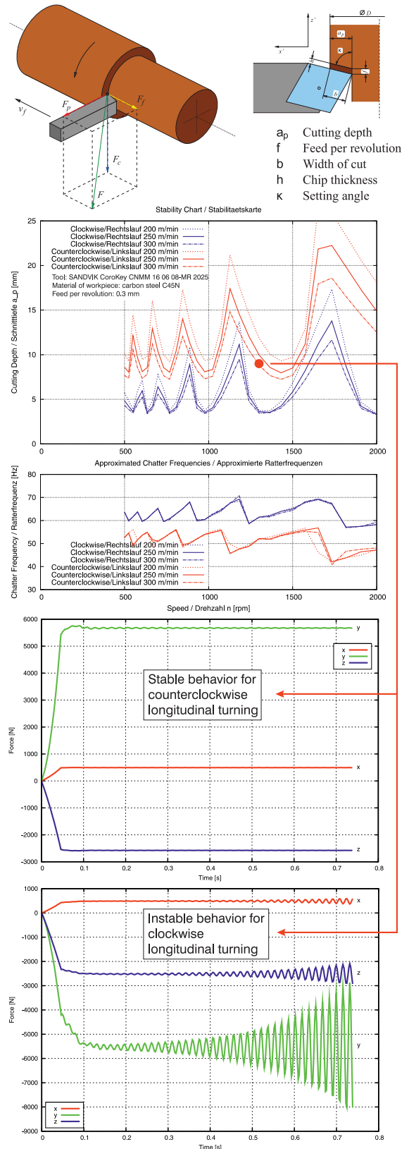
Figure 46: Stability chart for longitudinal turning with stable and instable behaviour under counterclockwise and clockwise turning.
