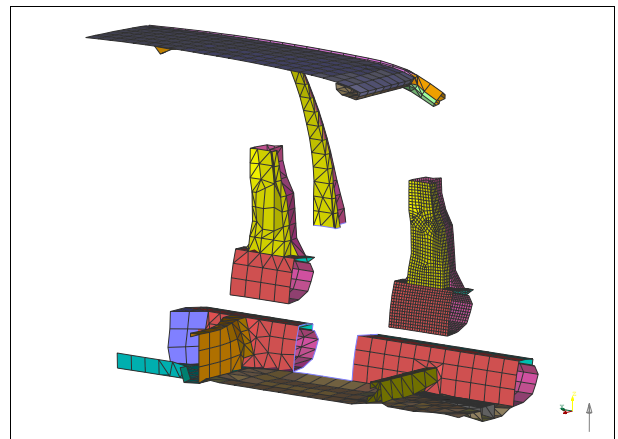
Figure 80: Application of local mesh refinement
