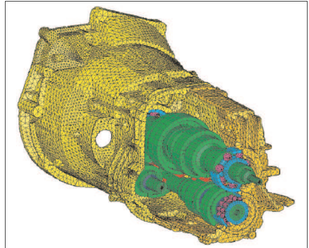
Figure 103: Bearing housing ZF AG
