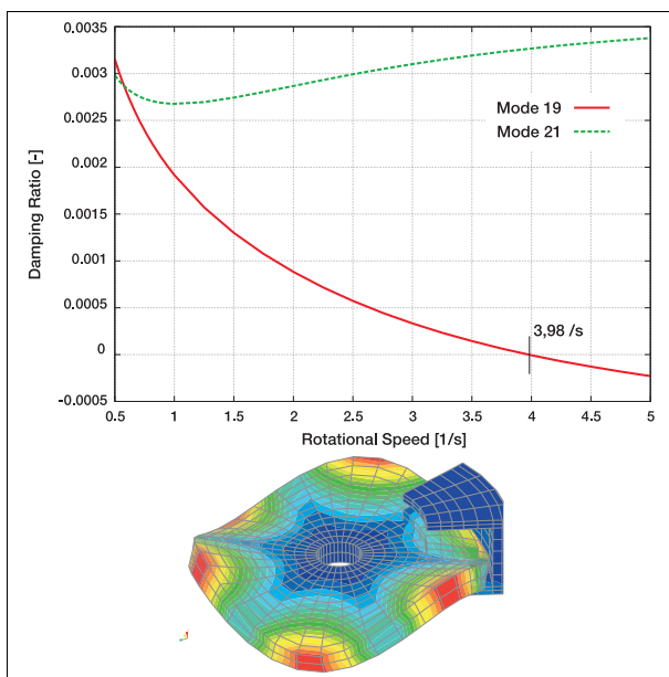
Figure 36: Simple brake model (2) with an unstable bending mode ( m=3, n=1 ) at 3,98 rps
