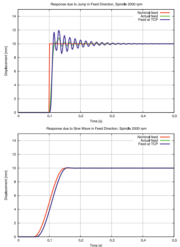
Figure 45: Time-history response due to excitation in Z direction for a sudden position jump (above) and a smooth position change (below) for the controlled machine
