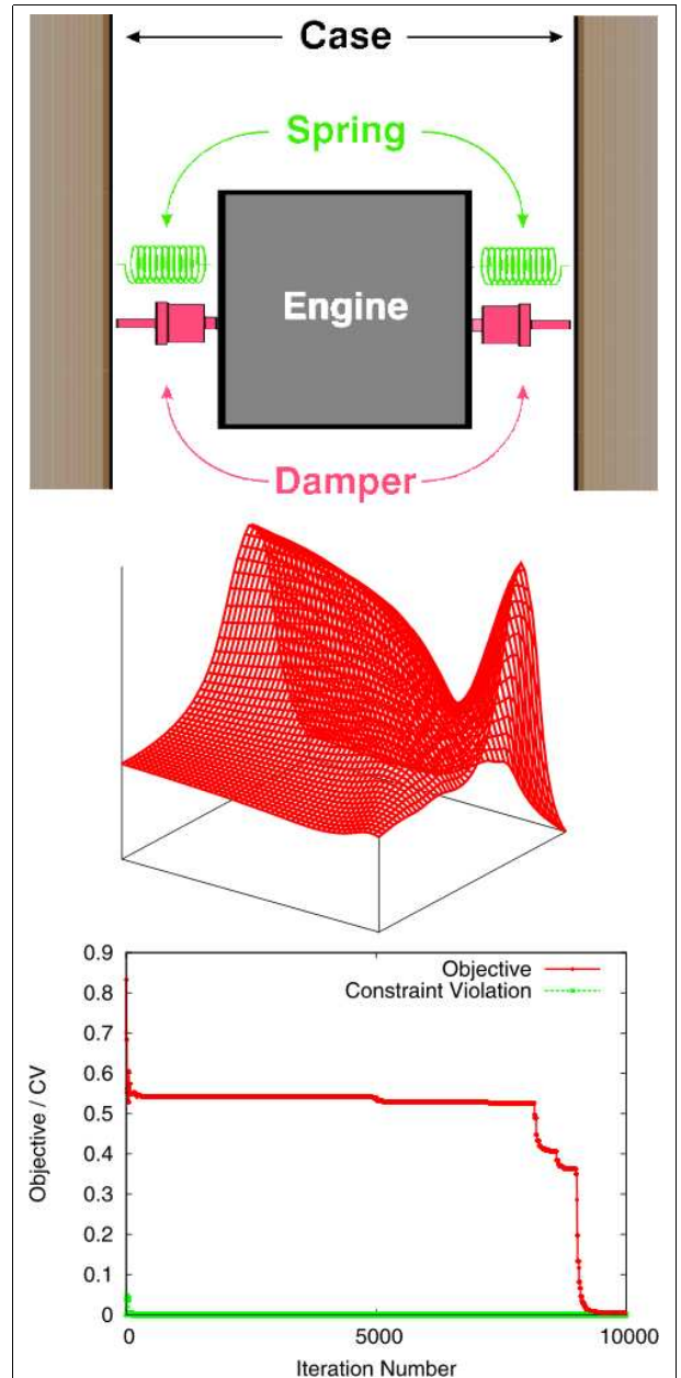
Figure 147: Global optimization of a spring-damper system with the LDR method. Top: model with 4 design variables, Middle: 2 design variables fixed at the optimum, objective function dependent on the 2 free variables, Bottom: course of objective function and constraint violation during the iterations.
