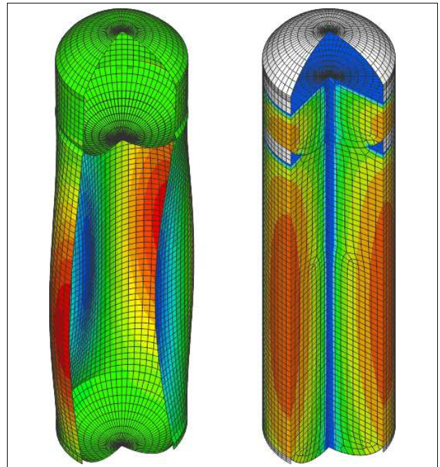
Figure 133: A coupled vibration mode shape of a fluid-filled space tank with corresponding pressure mode
