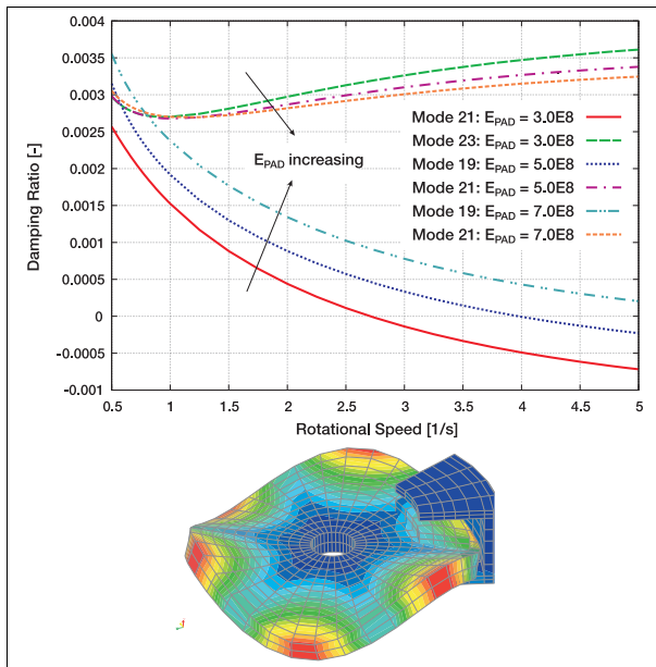
Figure 38: Simple brake model (4)
