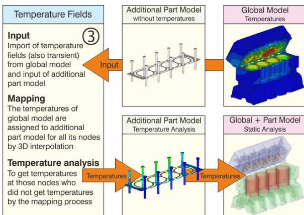
Figure 74: Mapping with extrapolation of temperature fields
