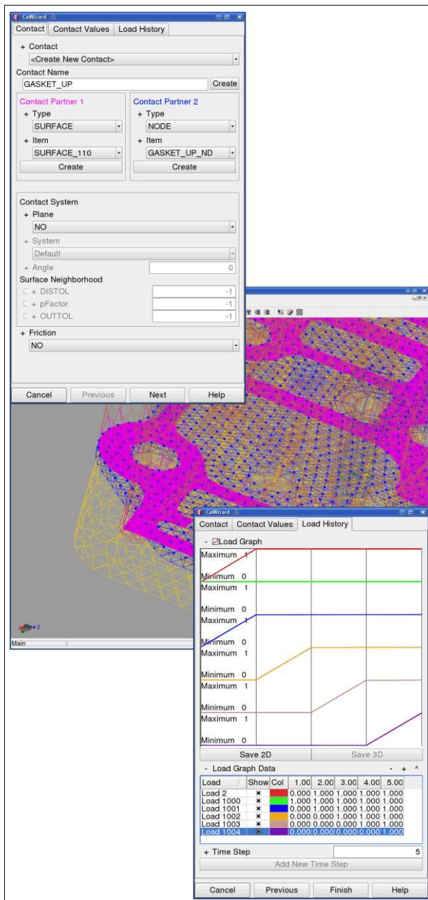
Figure 64: Contact modeling Contact topology and load history definition
