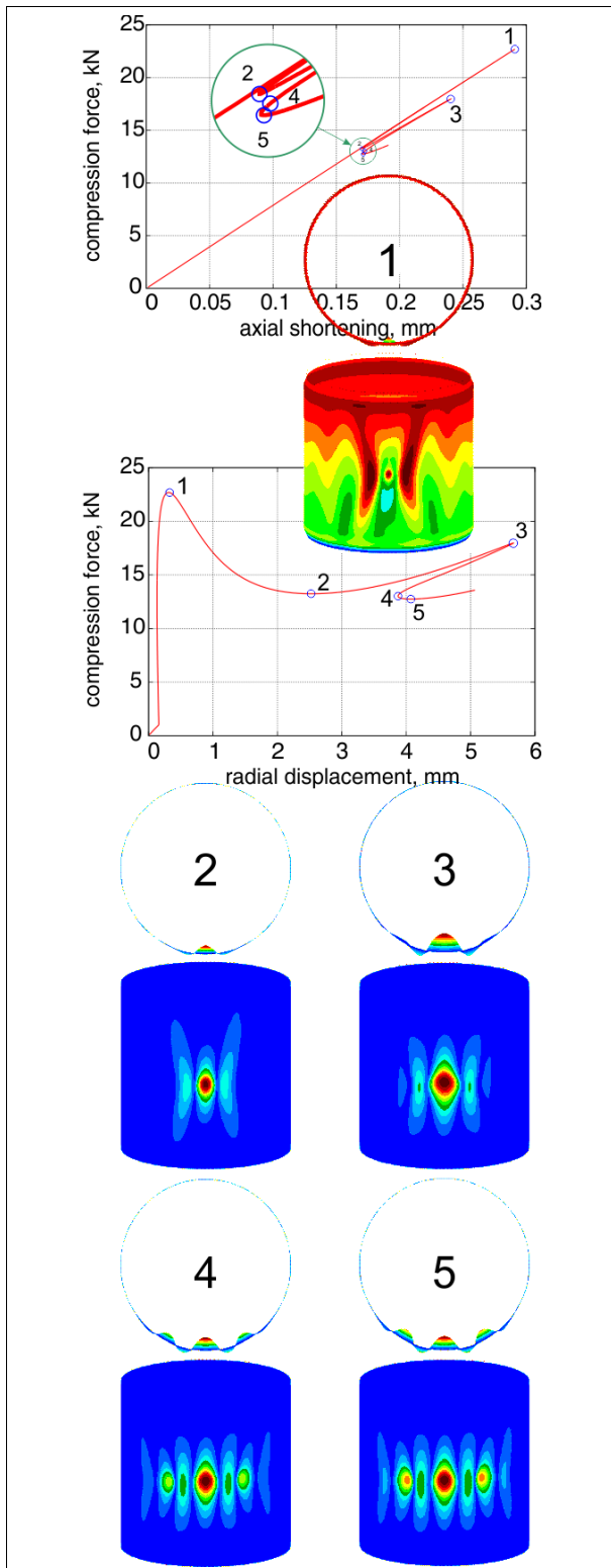
Figure 14: Nonlinear buckling with post-buckling behavior for a laminated cylinder shell
