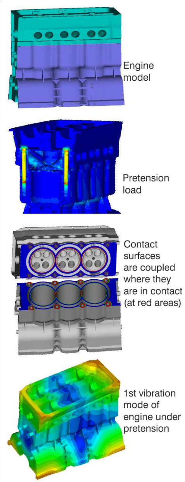
Figure 31: Dynamic analysis of an engine under pretension load
