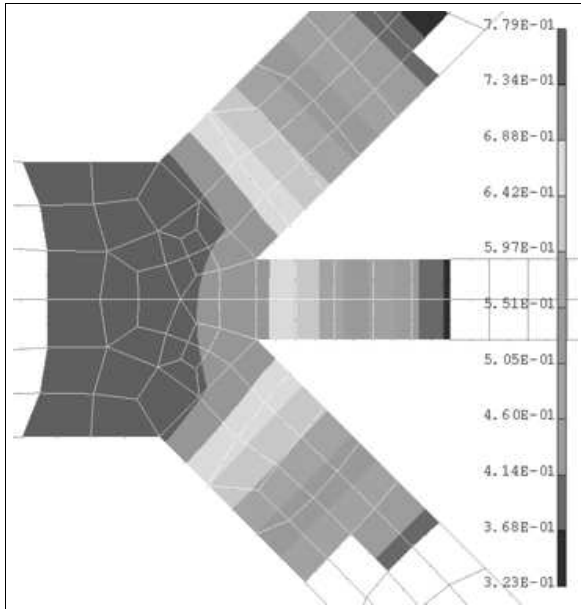
Figure 150: Scalar potential in an electric junction
