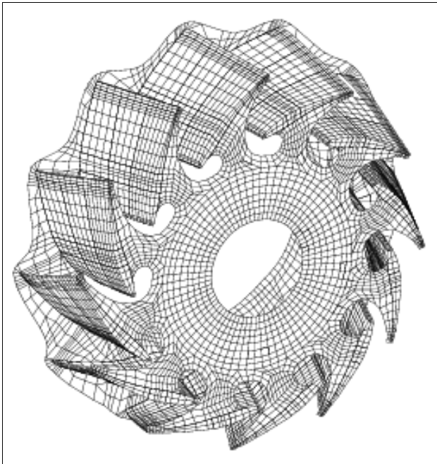
Figure 123: Half Model of a Turbine Half Model of a Turbine, 8th Mode Shape with Antisymmetric Boundary Conditions
