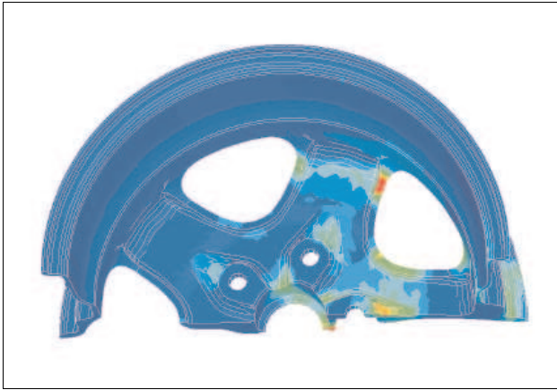
Figure 118: Impact test of a wheel with effective plastic strain.
