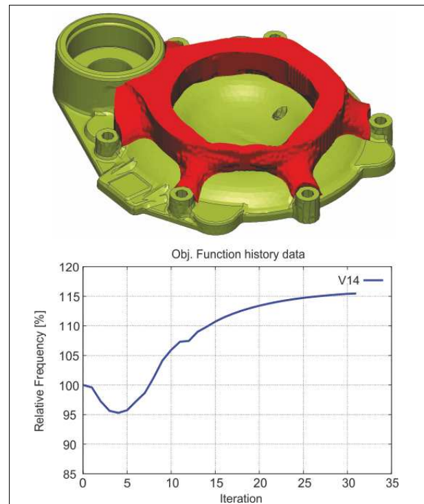
Figure 141: Topology optimization of a gearbox cover to maximize the second eigenfrequency with release direction (by courtesy of ZF Friedrichshafen AG)
