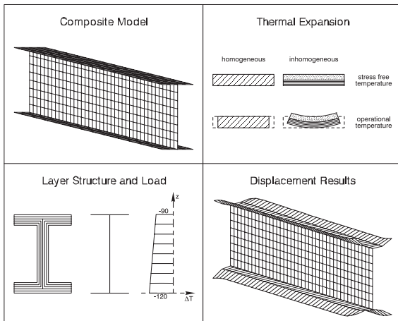
Figure 148: Laminate analysis of a girder
