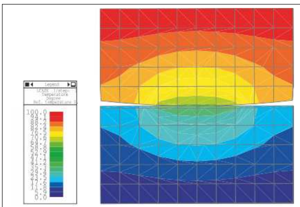
Figure 109: Temperature distribution in two contacting bodies
