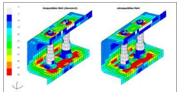
Figure 81: Results for part assembly with compatible (left) and incompatible (right) mesh
