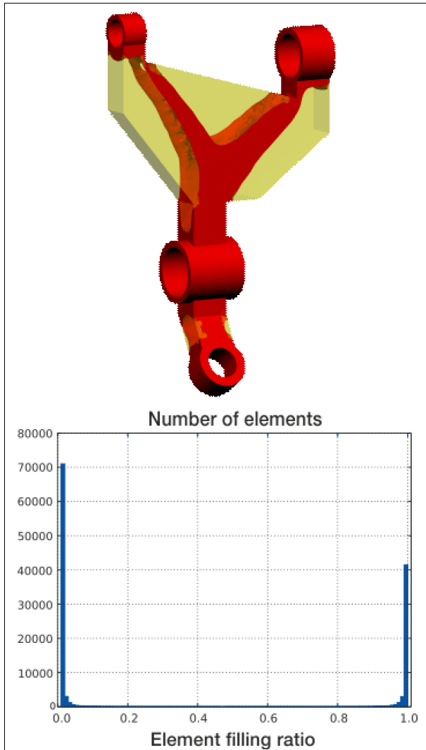
Figure 142: Fully converged topology
