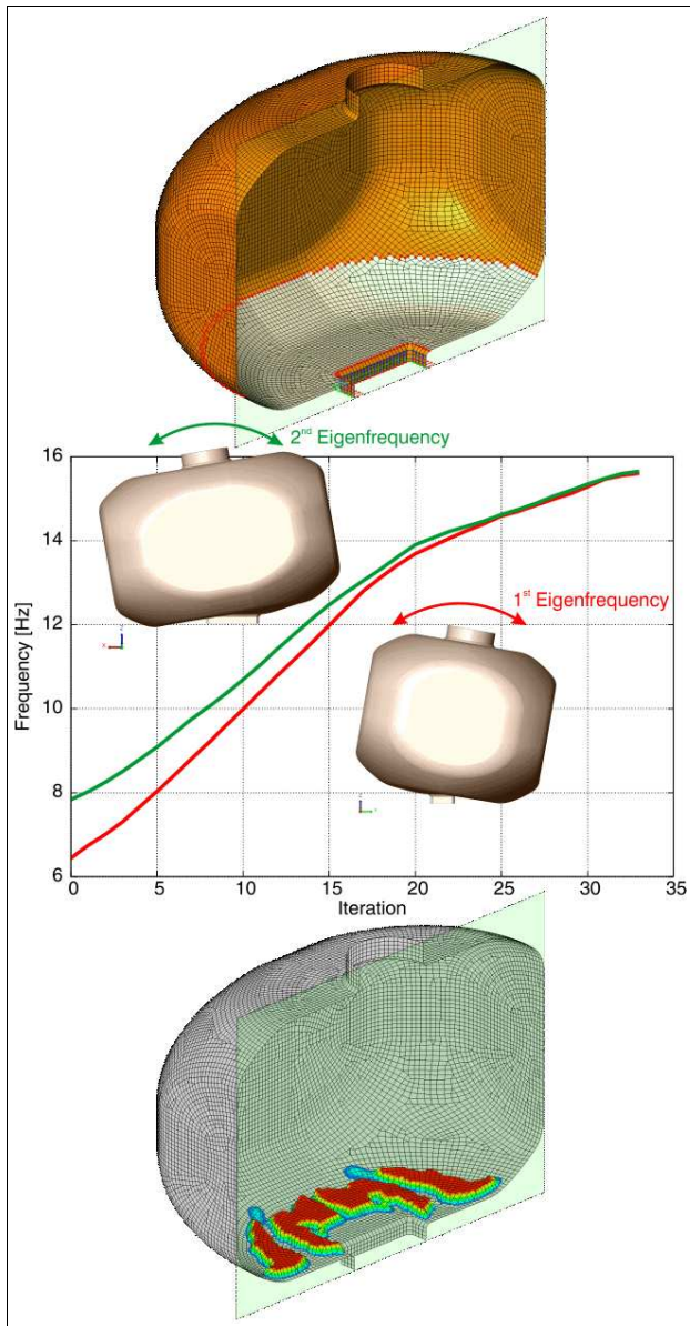
Figure 136: Bead generation for plastic tank
