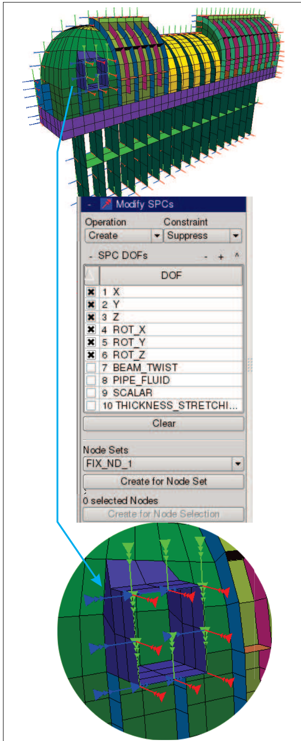
Figure 56: Specifying single point constraints
