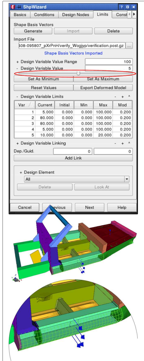
Figure 60: Definition of shape basis vectors of a car sill. The shape changes can be visualized by moving the slider in the menu.
