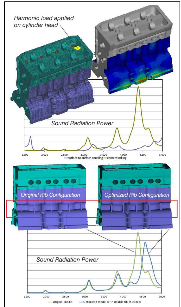
Figure 32: Optimization of rib thickness and rib position to reduce sound radiation from engine block surface
