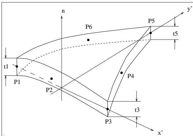
Figure 90: Triangular element with curved edges
