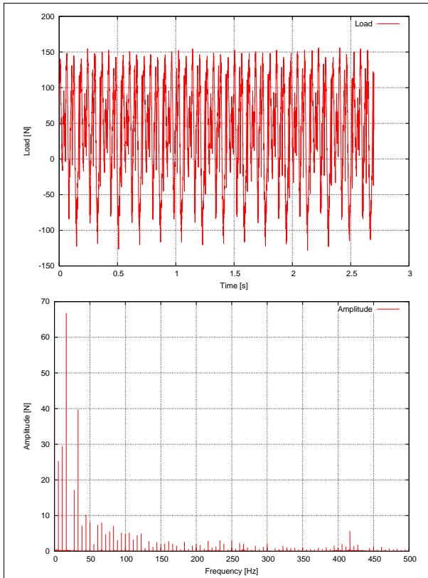
Figure 95: Example for the transformation of a periodic load (above in time domain, below in frequency domain)
