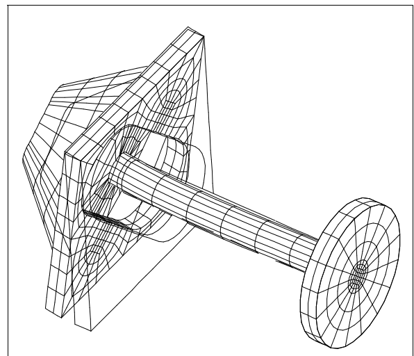
Figure 100: Clutch Element, Static Displacements
