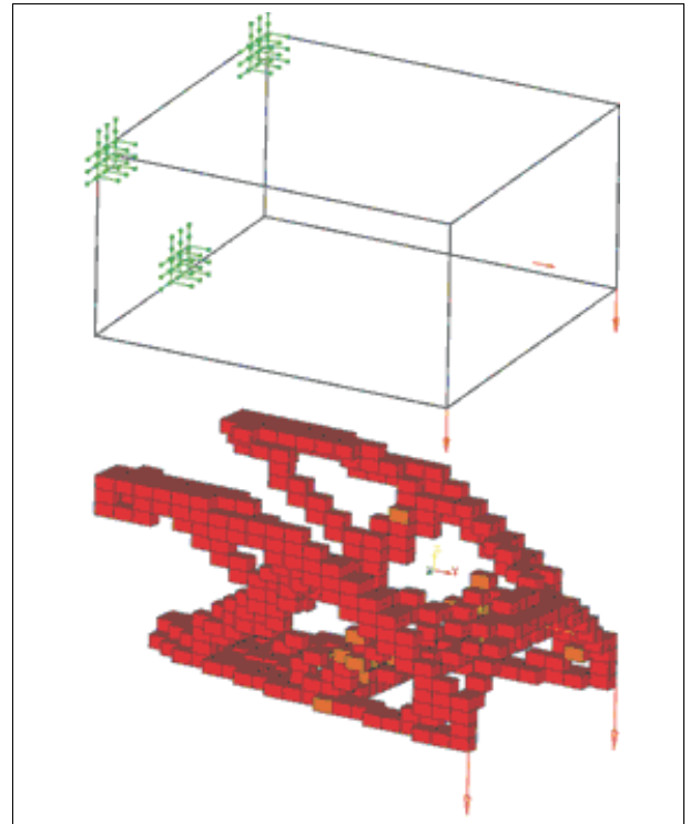
Figure 139: Layout optimization Design space with boundary conditions and loading (above) and the optimal material distribution (below)
