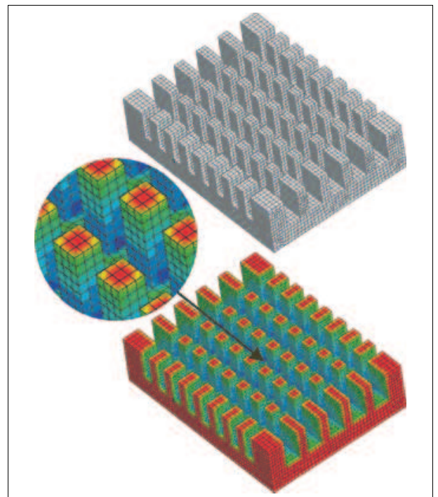
Figure 121: Analysis of cooling element with radiation
