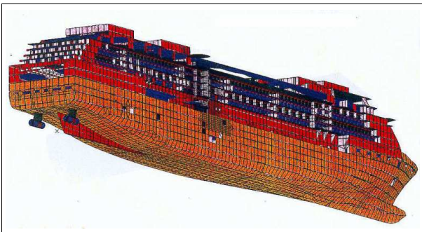
Figure 132: Ship model
