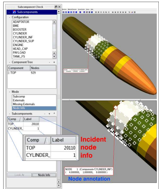
Figure 67: Visualization of coupling nodes of a substructure model
