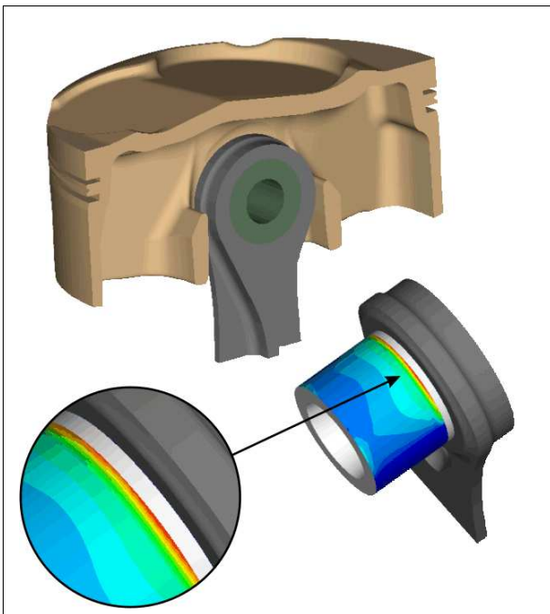
Figure 145: Optimization of contact pressure between piston and piston pin (Mahle GmbH, Stuttgart). The figure shows the edge pressure between both parts (for the optimized result see also next Fig. 146).
