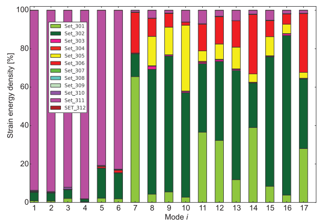
Figure 124: Analysis of strain energy density in element sets and for various modes
