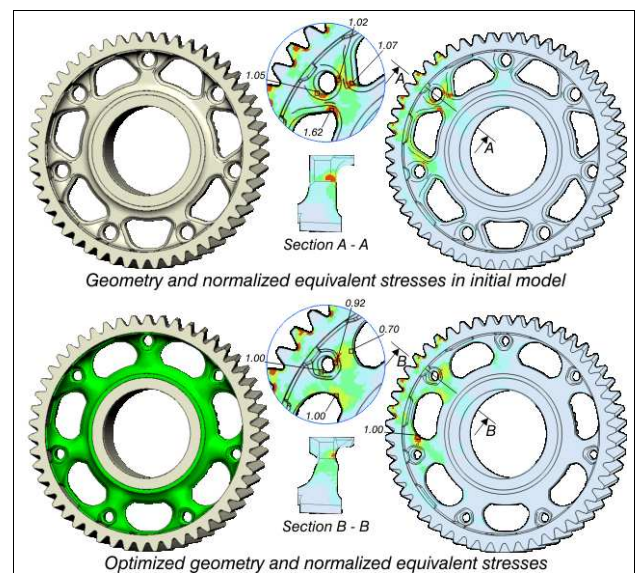
Figure 59: Shape optimization of a gearwheel Definition of cyclic symmetry, max. stress, minimum weight as objective function (by courtesy of Daimler AG, Stuttgart).
