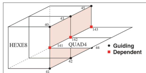
Figure 88: MPC example: Volume Shell Transition
