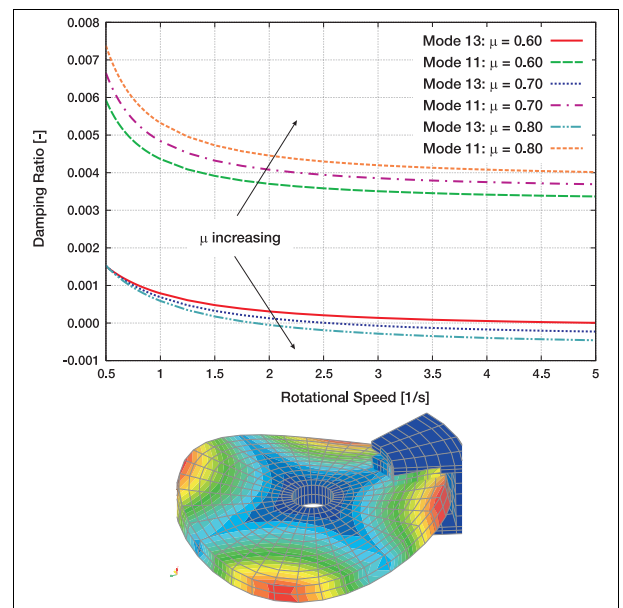
Figure 37: Simple brake model (3) with an unstable bending mode ( m=2, n=1 ) which becomes unstable at different rotational speeds dependent on the frictional coefficient.
