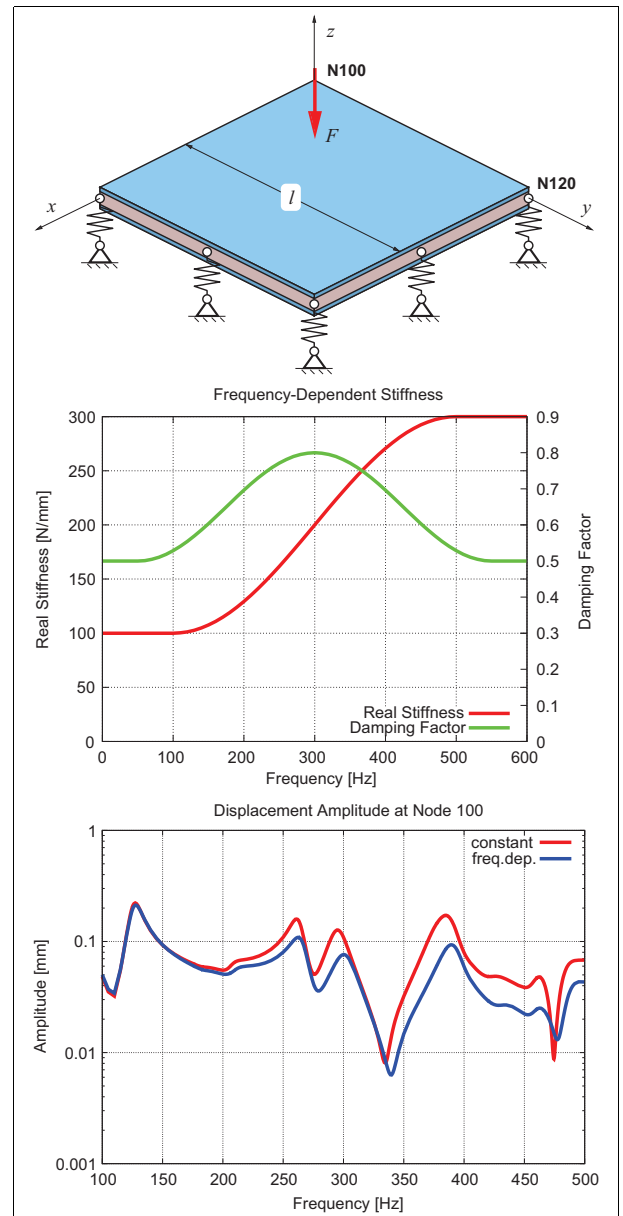
Figure 128: Frequency-dependent stiffness and frequency dependent viscous damping in frequency response analysis
