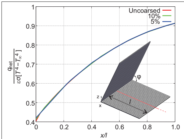
Figure 122: Heat radiation between adjoint plates
